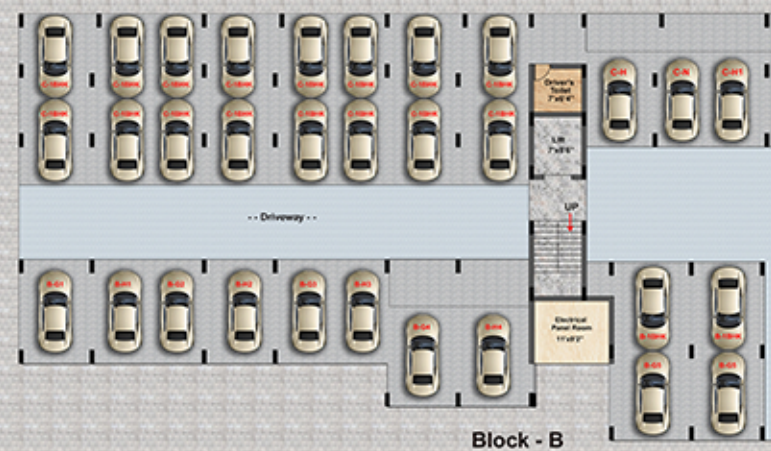
STILT FLOOR PLAN - BLOCK . B
