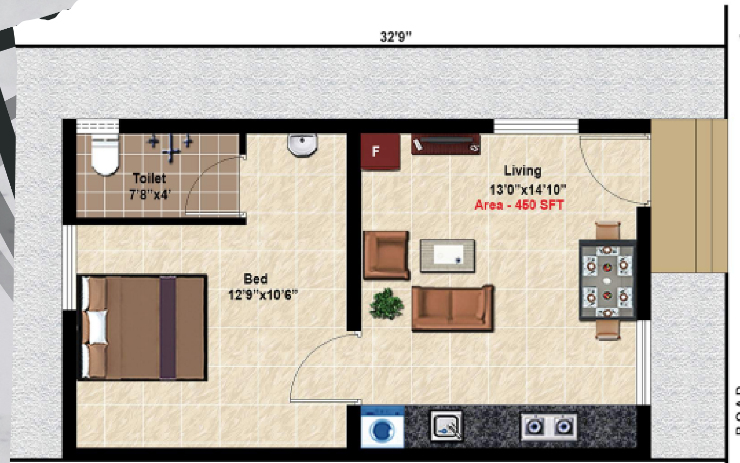
Site Cum Ground Floor Plan 1BHK - Individual Villa - East Facing
